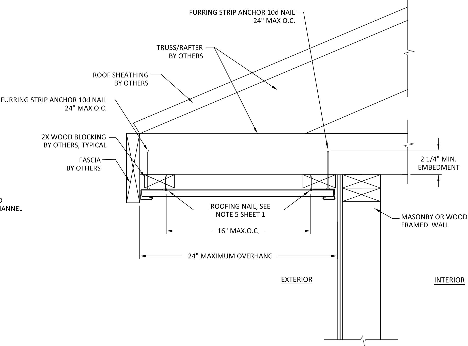
A 2 VERTICAL SECTION SOFFIT INSTALLATION DETAIL 2X WOOD FRAMING OR 1X FURRING STRIP
